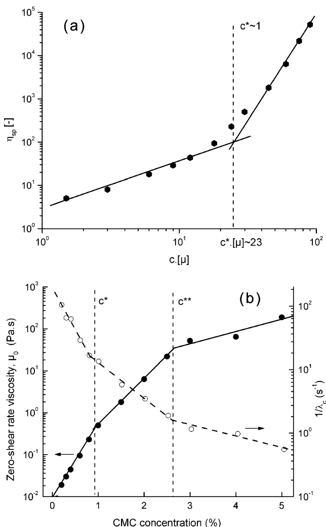
Fig. 2 a Overlap parameter, c.[\mu] , as a function of specific viscosity, \mu_{sp} , at different concentrations of CMC solutions. b The reciprocal of the time constant, 1/\lambda_c , and the zero shear rate viscosity, \mu_0 , as a function of CMC concentration
