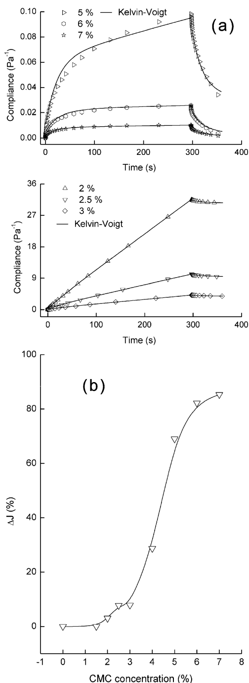
Fig. 4 a Creep recovery curves of CMC solutions at different concentrations. b Variation of the elastic recovery index \Delta J as a function of CMC concentration
